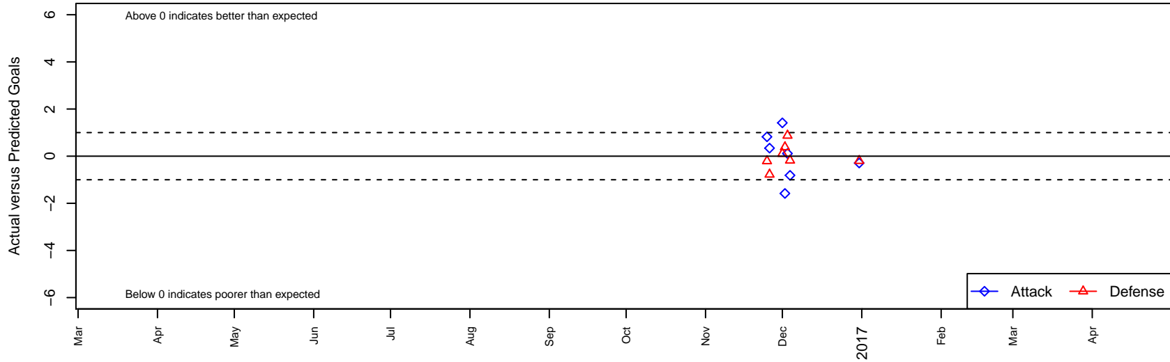
NJ Stallions Stampede G00 Dots are actual minus expected GF (blue circles) and GA (red triangles). Blue line is smoothed change in attack strength. Red is smoothed change in defense strength.
